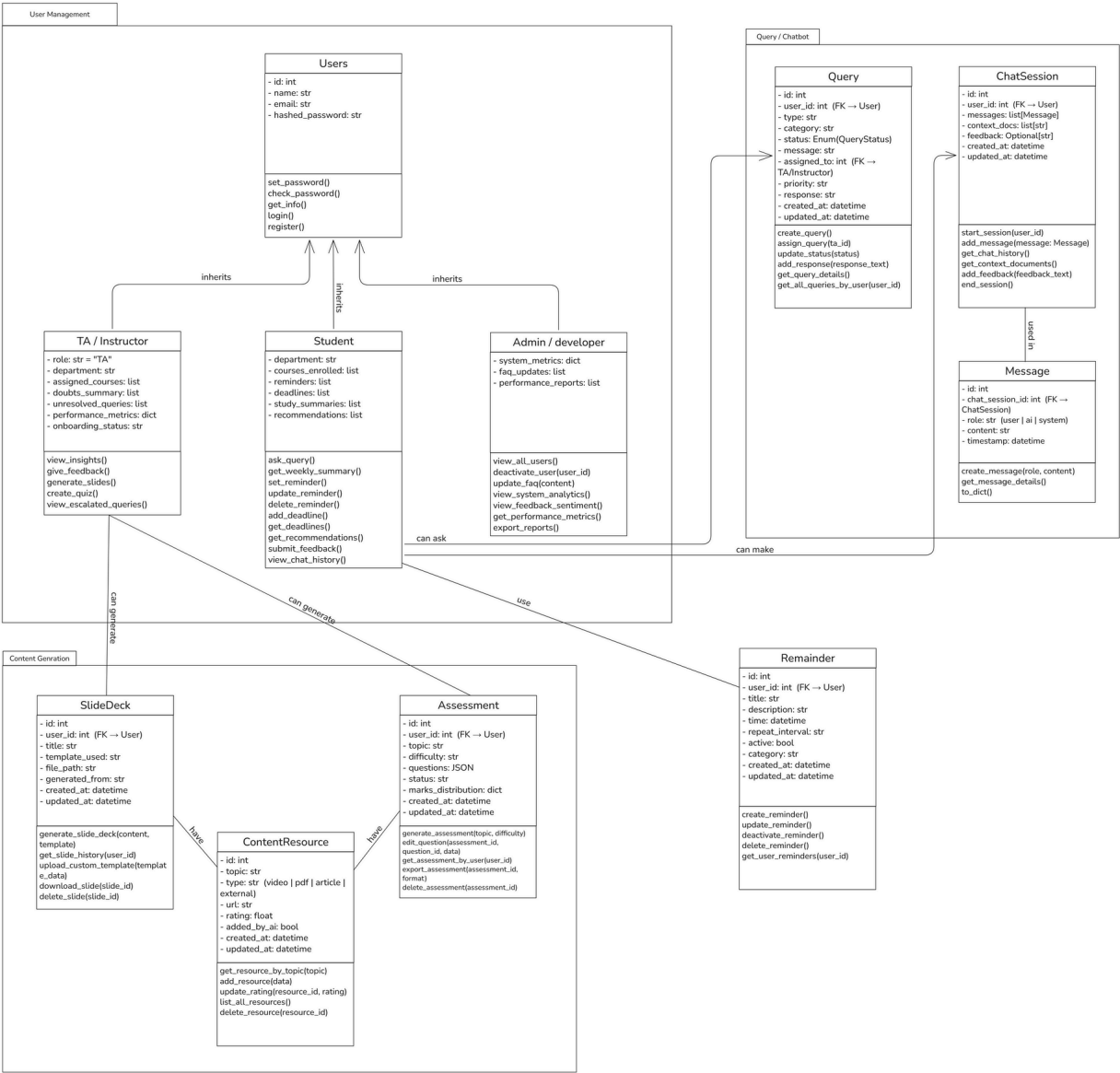
Class Diagram
